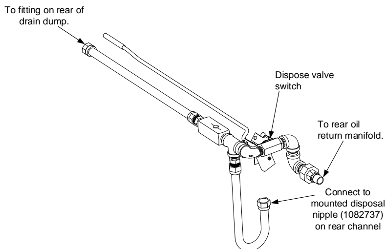
Figure 7: Rear View of Rear Oil Assembly
